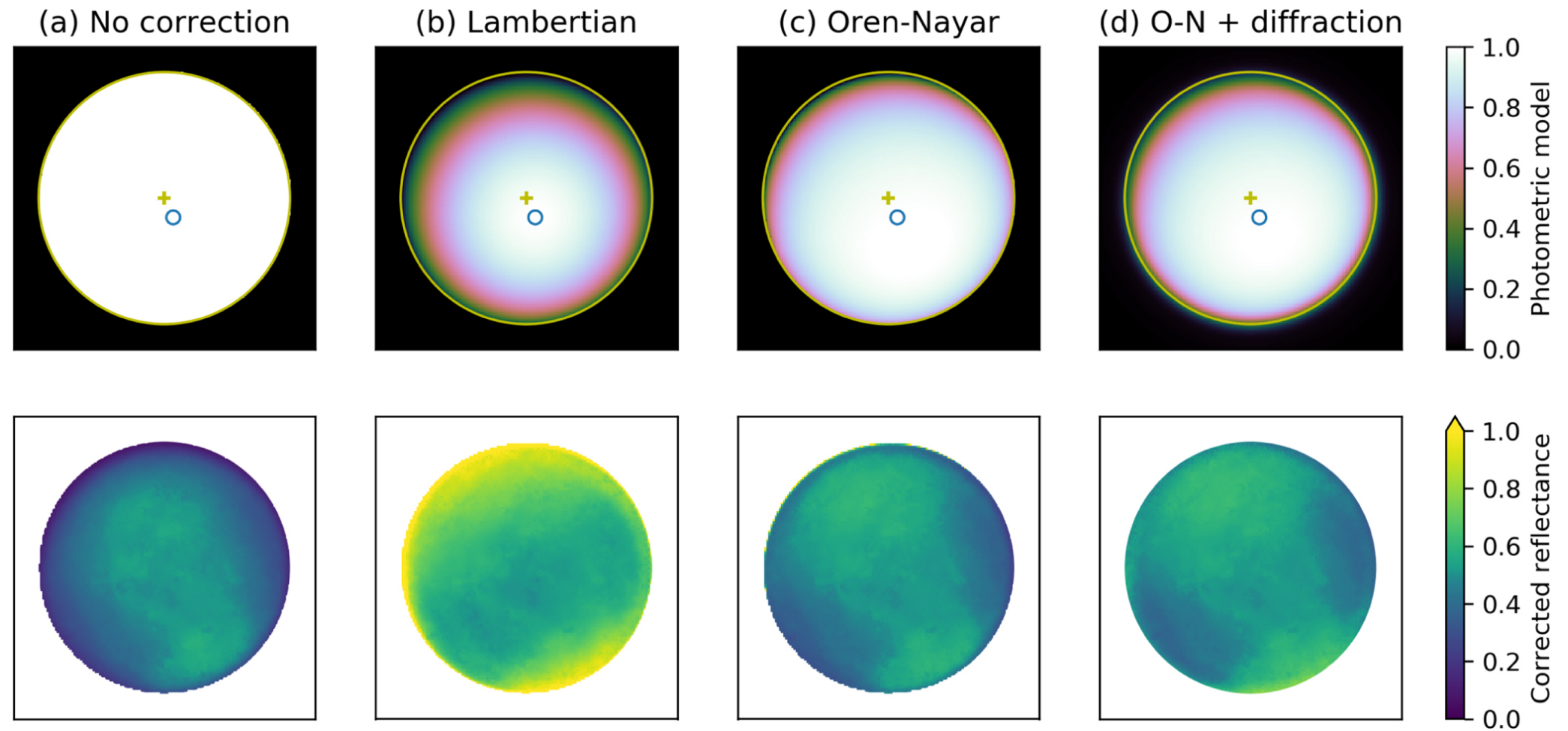
Figure 4. from Oliver King et al 2022 Planet. Sci. J. 3 doi:10.3847/PSJ/ac596d https://dx.doi.org/10.3847/PSJ/ac596d © 2022. The Author(s). Published by the American Astronomical Society.
