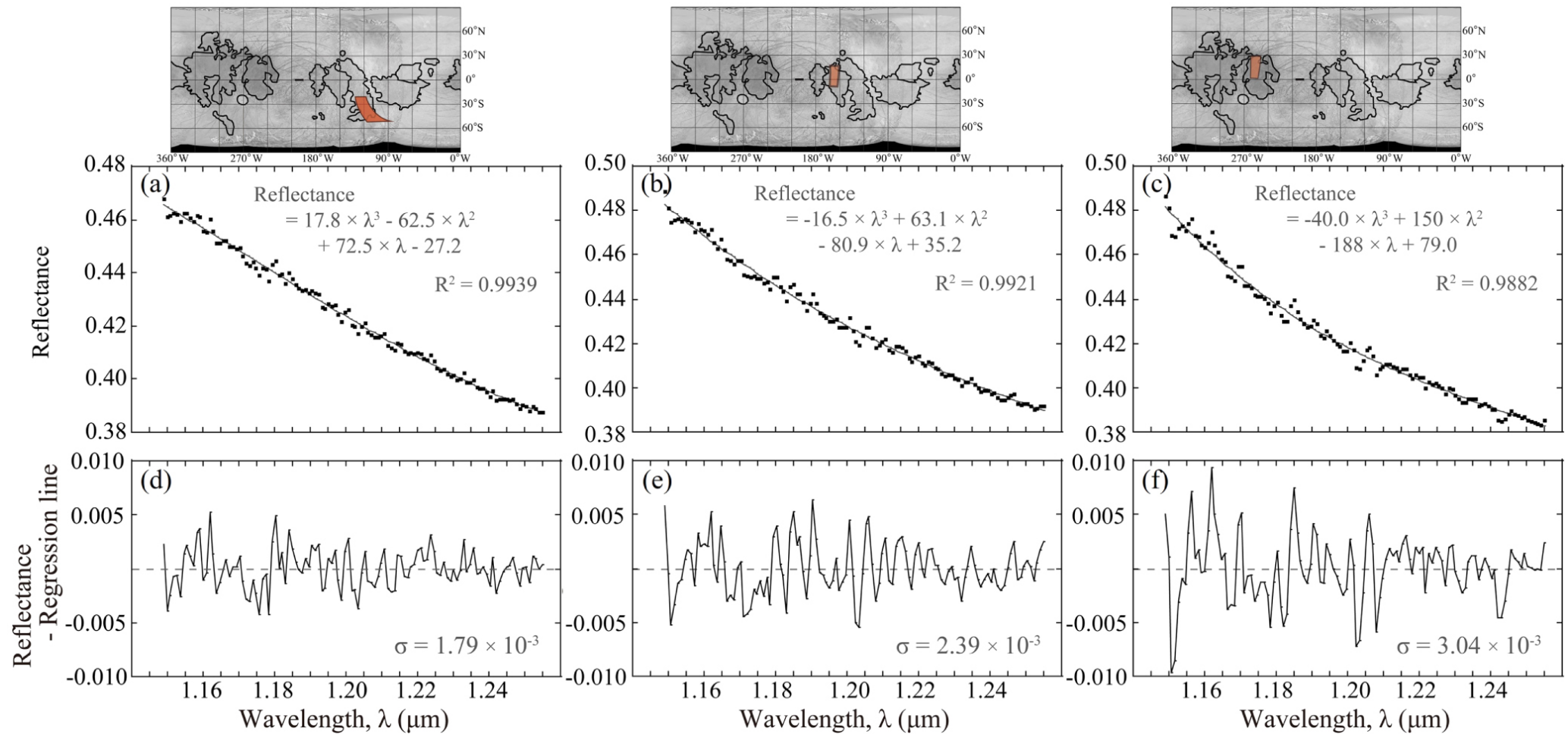
Figure 9. from Shuya Tan et al 2022 Planet. Sci. J. 3 doi:10.3847/PSJ/ac596c https://dx.doi.org/10.3847/PSJ/ac596c © 2022. The Author(s). Published by the American Astronomical Society.
