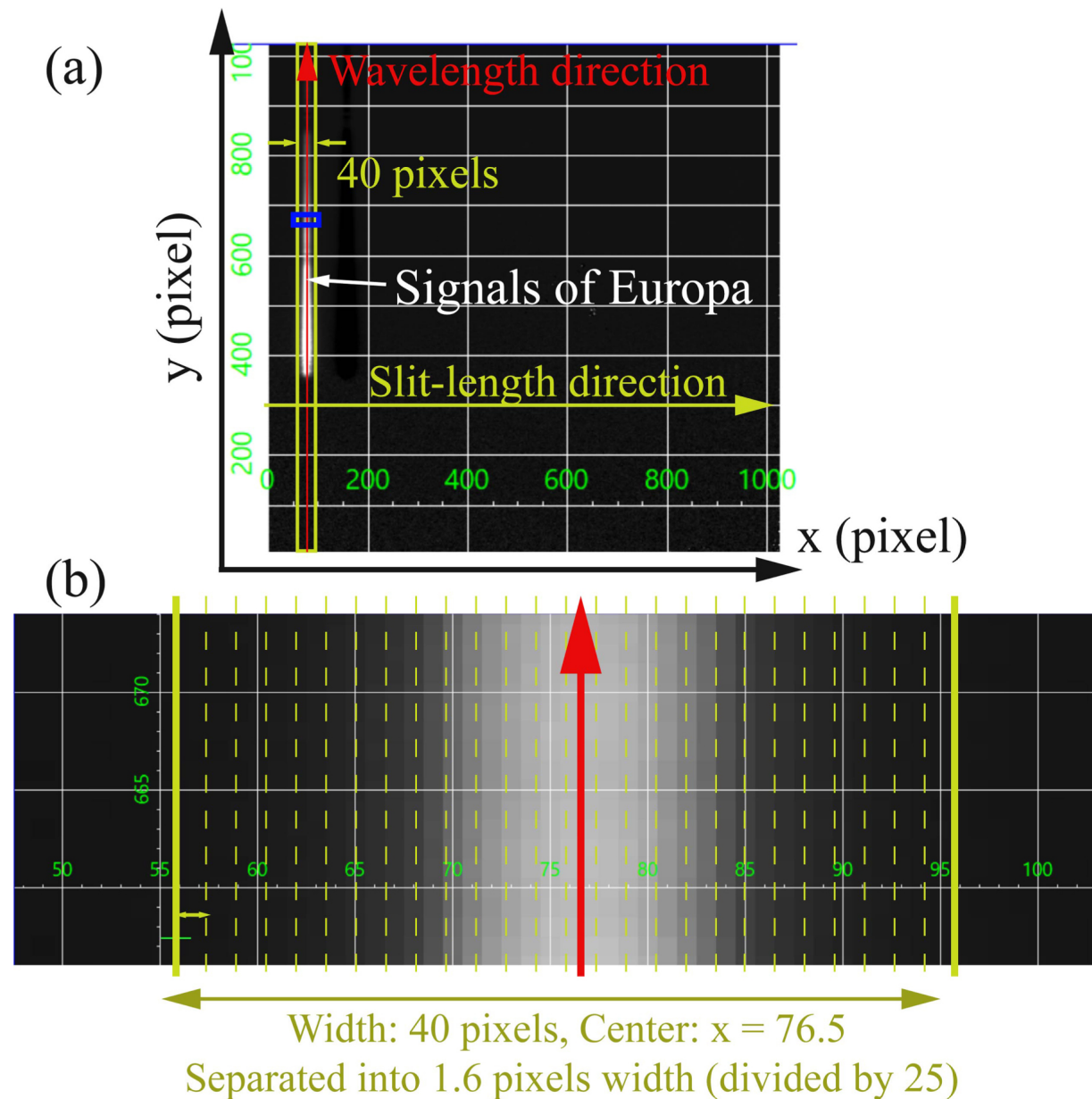
Figure 3. from Shuya Tan et al 2022 Planet. Sci. J. 3 doi:10.3847/PSJ/ac596c https://dx.doi.org/10.3847/PSJ/ac596c © 2022. The Author(s). Published by the American Astronomical Society.
