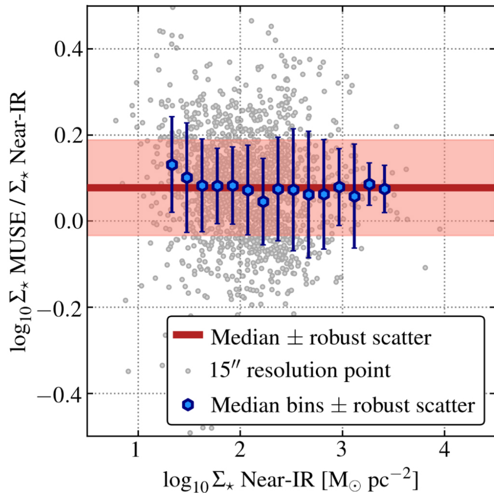
Figure 8. from Adam K. Leroy et al 2021 Astrophys. J. Suppl. 257 doi:10.3847/1538-4365/ac17f3 https://dx.doi.org/10.3847/1538-4365/ac17f3 © 2021. The American Astronomical Society. All rights reserved.
