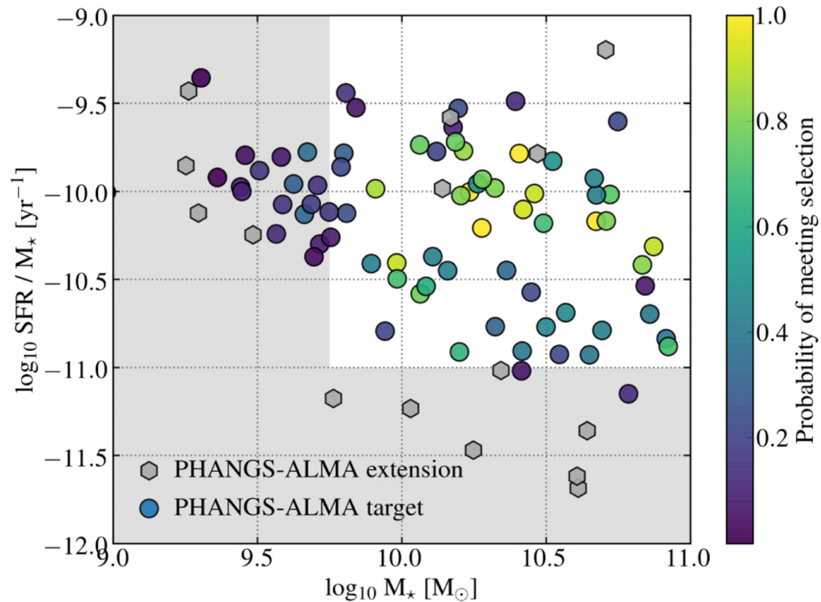
Figure 7. from Adam K. Leroy et al 2021 Astrophys. J. Suppl. 257 doi:10.3847/1538-4365/ac17f3 https://dx.doi.org/10.3847/1538-4365/ac17f3 © 2021. The American Astronomical Society. All rights reserved.
