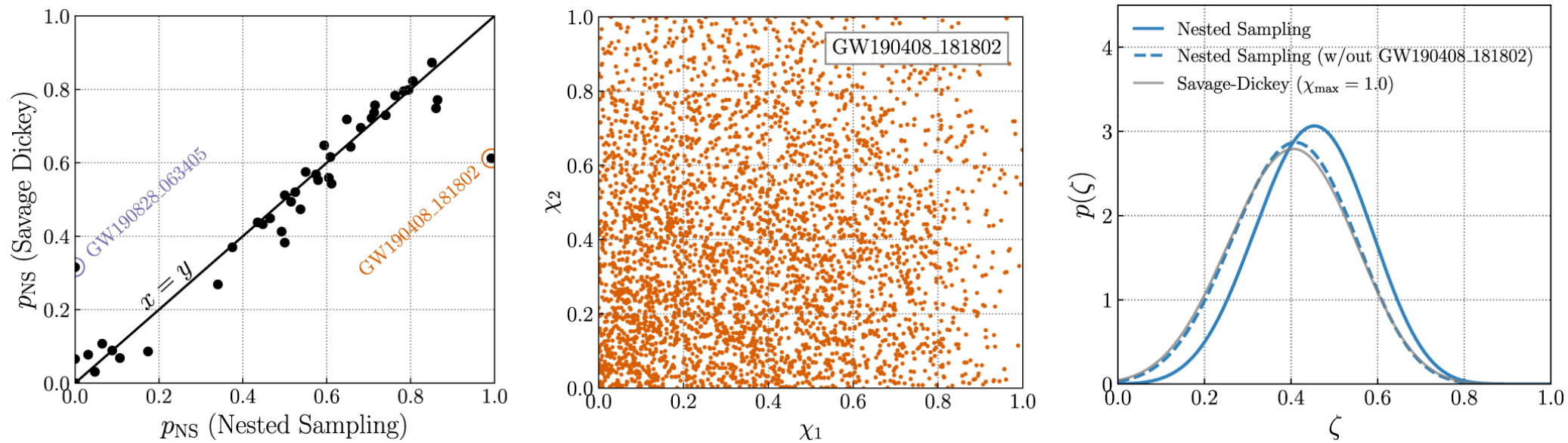
Figure 14. from Thomas A. Callister et al 2022 Astrophys. J. Lett. 937 doi:10.3847/2041-8213/ac847e https://dx.doi.org/10.3847/2041-8213/ac847e © 2022. The Author(s). Published by the American Astronomical Society.
