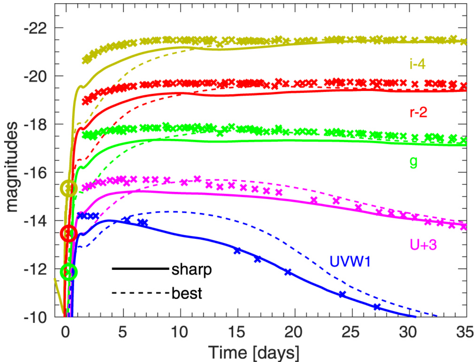
Figure 7. from Alexandra Kozyreva et al 2022 Astrophys. J. Lett. 934 doi:10.3847/2041-8213/ac835a https://dx.doi.org/10.3847/2041-8213/ac835a © 2022. The Author(s). Published by the American Astronomical Society.
