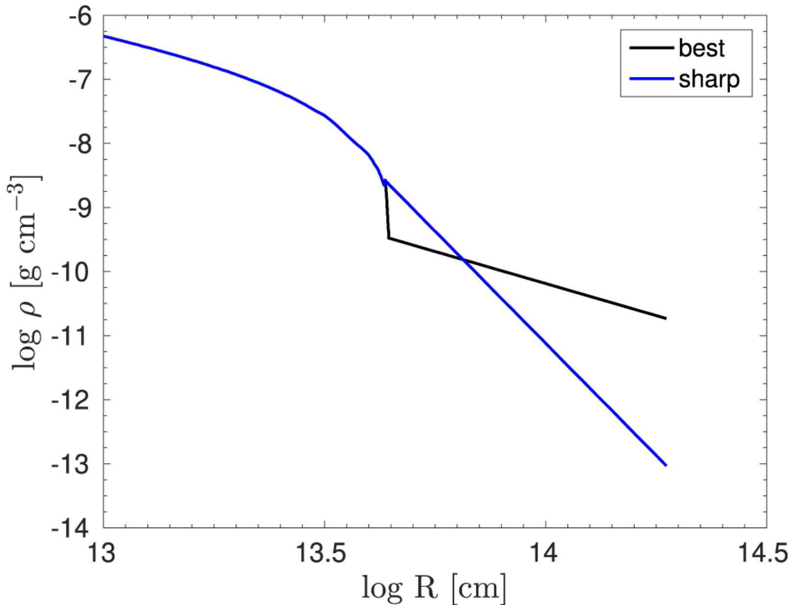
Figure 6. from Alexandra Kozyreva et al 2022 Astrophys. J. Lett. 934 doi:10.3847/2041-8213/ac835a https://dx.doi.org/10.3847/2041-8213/ac835a © 2022. The Author(s). Published by the American Astronomical Society.
