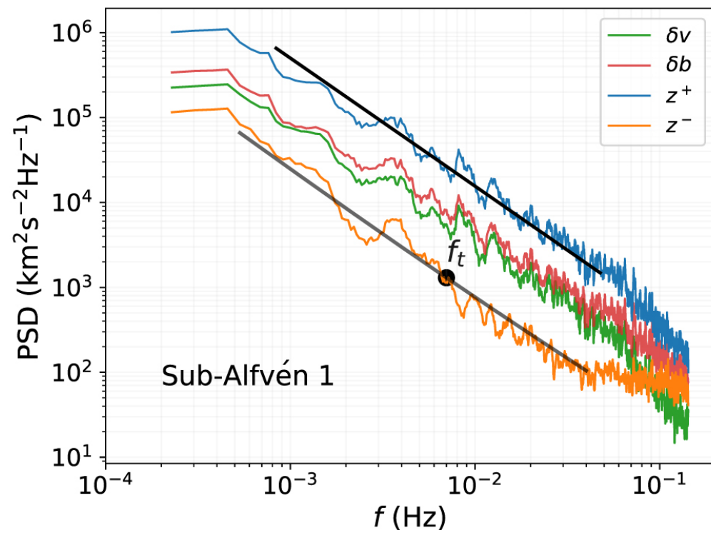
Figure 3. from L.-L. Zhao et al 2022 Astrophys. J. Lett. 934 doi:10.3847/2041-8213/ac8353 https://dx.doi.org/10.3847/2041-8213/ac8353 © 2022. The Author(s). Published by the American Astronomical Society.
