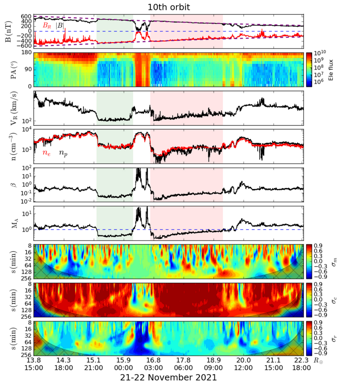
Figure 1. from L.-L. Zhao et al 2022 Astrophys. J. Lett. 934 doi:10.3847/2041-8213/ac8353 https://dx.doi.org/10.3847/2041-8213/ac8353 © 2022. The Author(s). Published by the American Astronomical Society.
