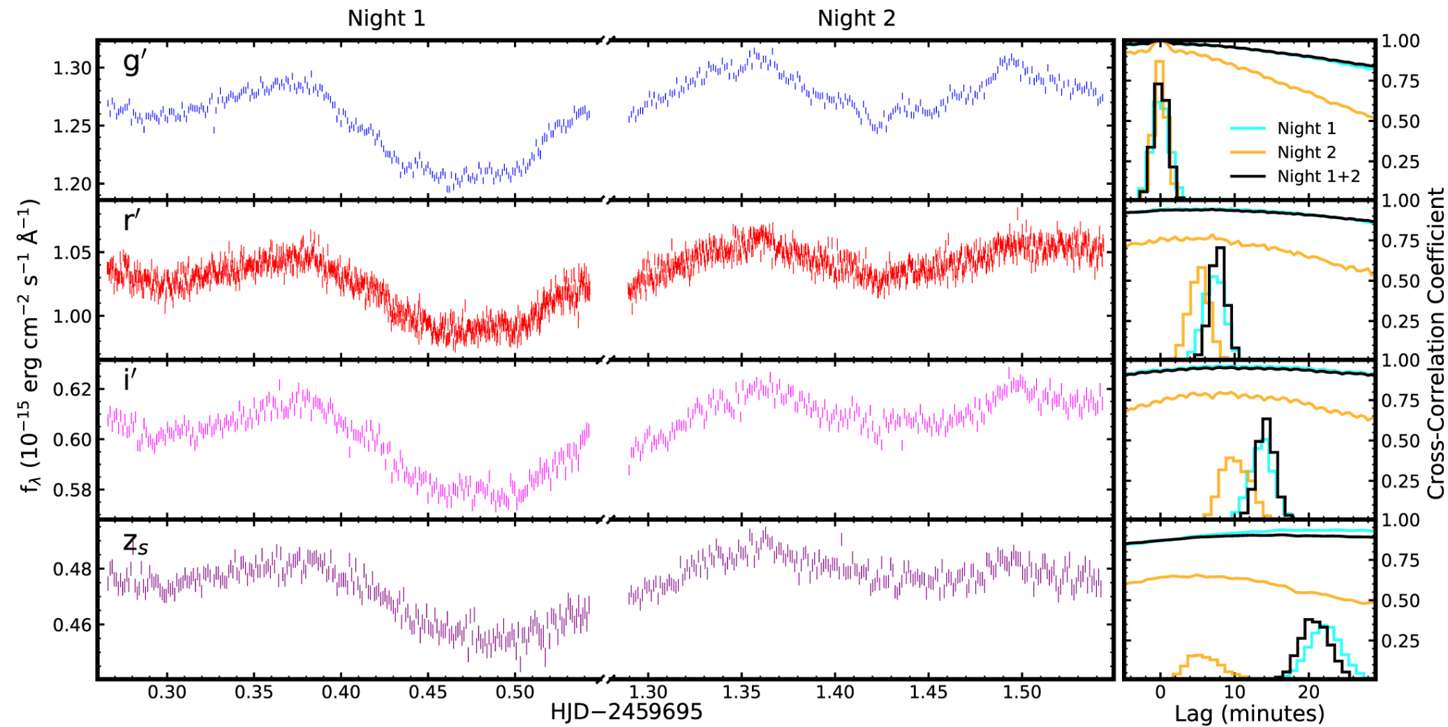
Figure 1. from John W. Montano et al 2022 Astrophys. J. Lett. 934 doi:10.3847/2041-8213/ac7e54 https://dx.doi.org/10.3847/2041-8213/ac7e54 © 2022. The Author(s). Published by the American Astronomical Society.
