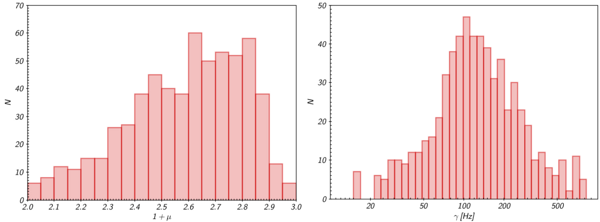
Figure 2. from High-frequency Magnetic Fluctuations in Space Plasmas and the Role of Electron Landau Damping null 2022 APJL 924 L26 doi:10.3847/2041-8213/ac4740 https://dx.doi.org/10.3847/2041-8213/ac4740 © 2022. The Author(s). Published by the American Astronomical Society.
