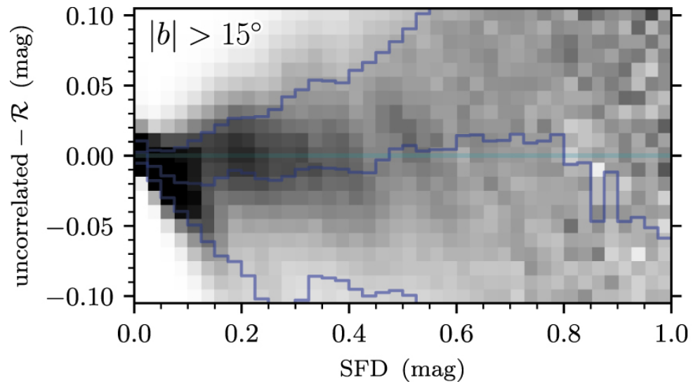
Figure 9. from A 3D Dust Map Based on Gaia, Pan-STARRS 1, and 2MASS null 2019 APJ 887 93 doi:10.3847/1538-4357/ab5362 http://dx.doi.org/10.3847/1538-4357/ab5362 © 2019. The American Astronomical Society. All rights reserved.
