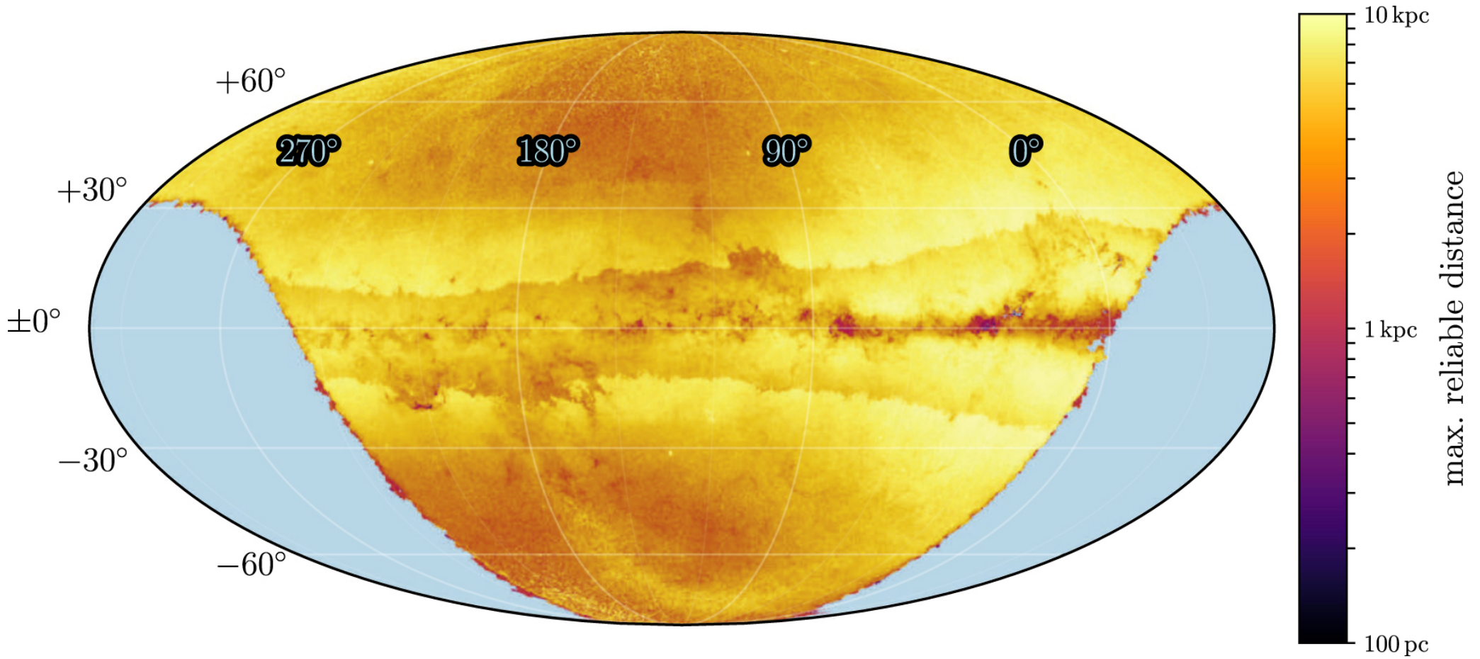
Figure 6. from A 3D Dust Map Based on Gaia, Pan-STARRS 1, and 2MASS null 2019 APJ 887 93 doi:10.3847/1538-4357/ab5362 http://dx.doi.org/10.3847/1538-4357/ab5362 © 2019. The American Astronomical Society. All rights reserved.
