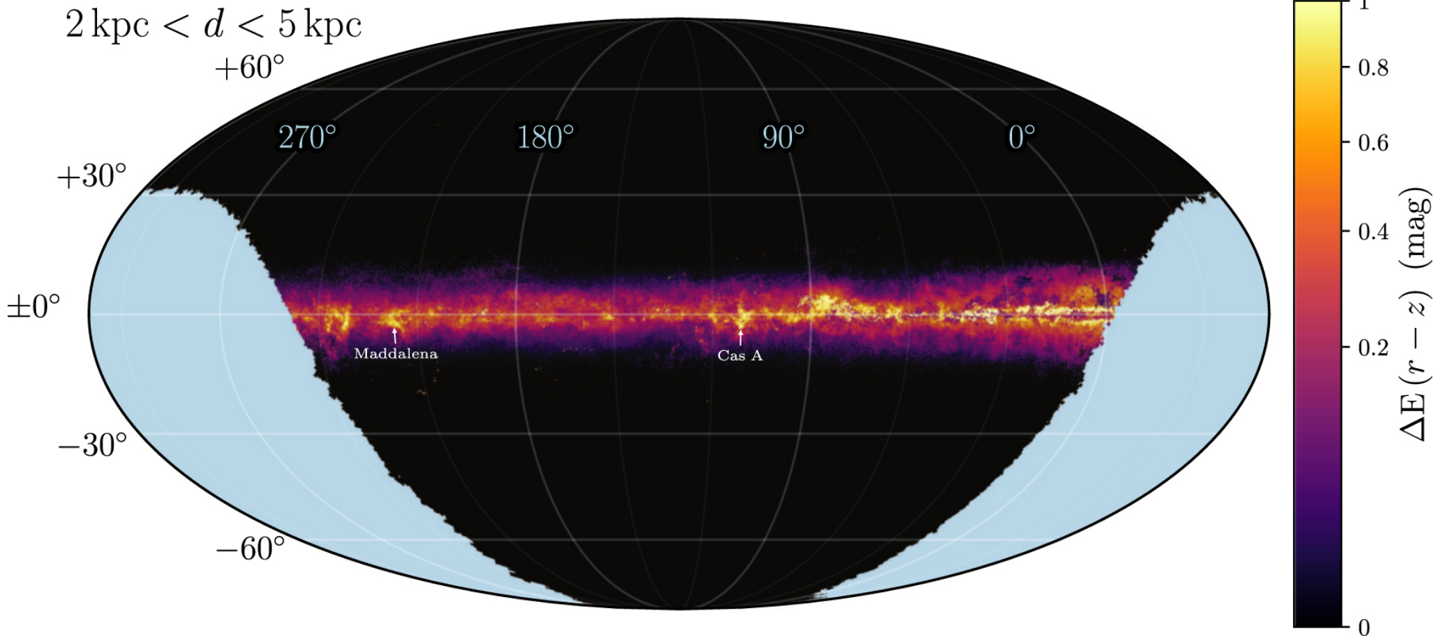
Figure 4. from A 3D Dust Map Based on Gaia, Pan-STARRS 1, and 2MASS null 2019 APJ 887 93 doi:10.3847/1538-4357/ab5362 http://dx.doi.org/10.3847/1538-4357/ab5362 © 2019. The American Astronomical Society. All rights reserved.
