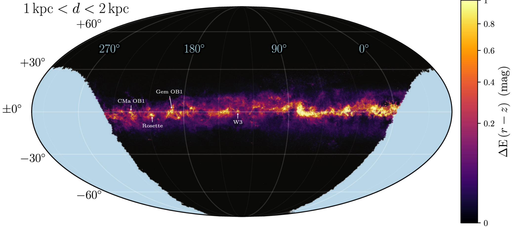
Figure 3. from A 3D Dust Map Based on Gaia, Pan-STARRS 1, and 2MASS null 2019 APJ 887 93 doi:10.3847/1538-4357/ab5362 http://dx.doi.org/10.3847/1538-4357/ab5362 © 2019. The American Astronomical Society. All rights reserved.
