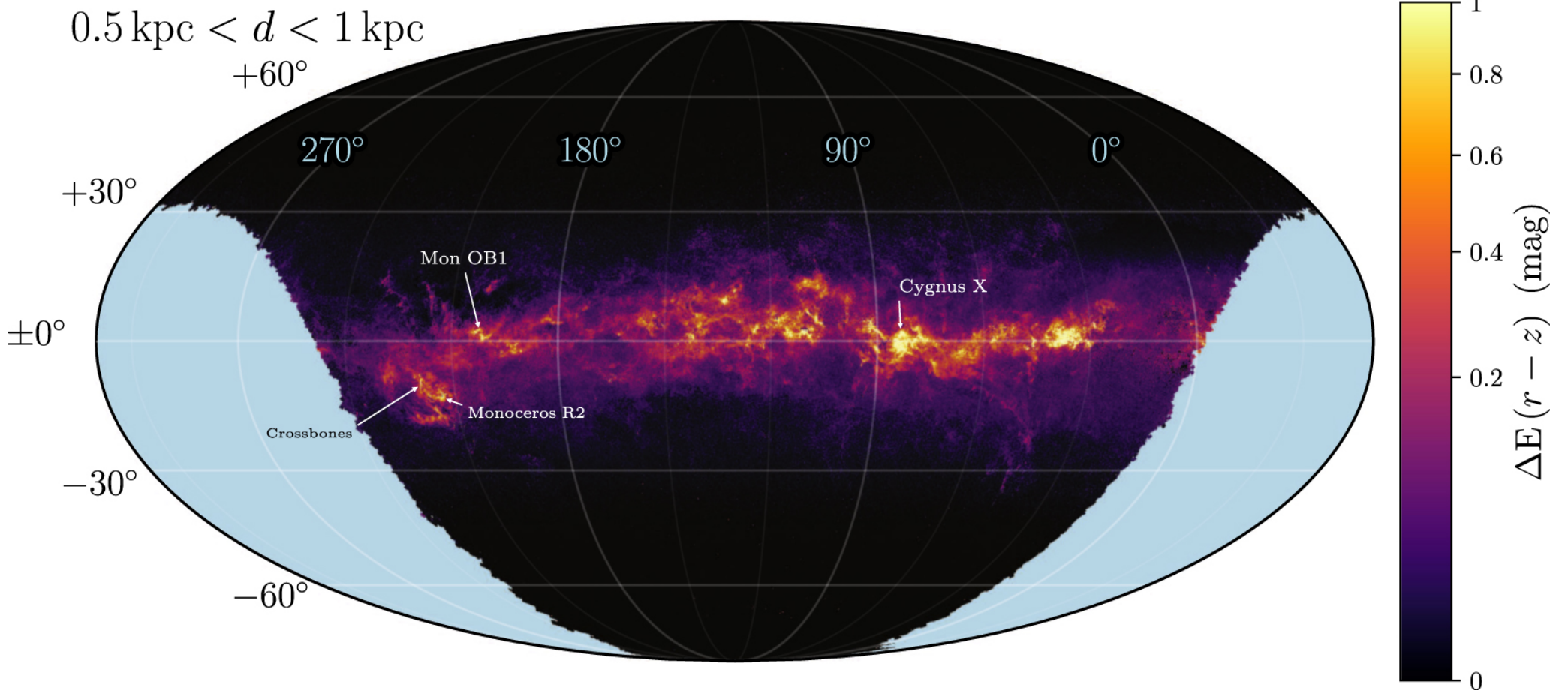
Figure 2. from A 3D Dust Map Based on Gaia, Pan-STARRS 1, and 2MASS null 2019 APJ 887 93 doi:10.3847/1538-4357/ab5362 http://dx.doi.org/10.3847/1538-4357/ab5362 © 2019. The American Astronomical Society. All rights reserved.
