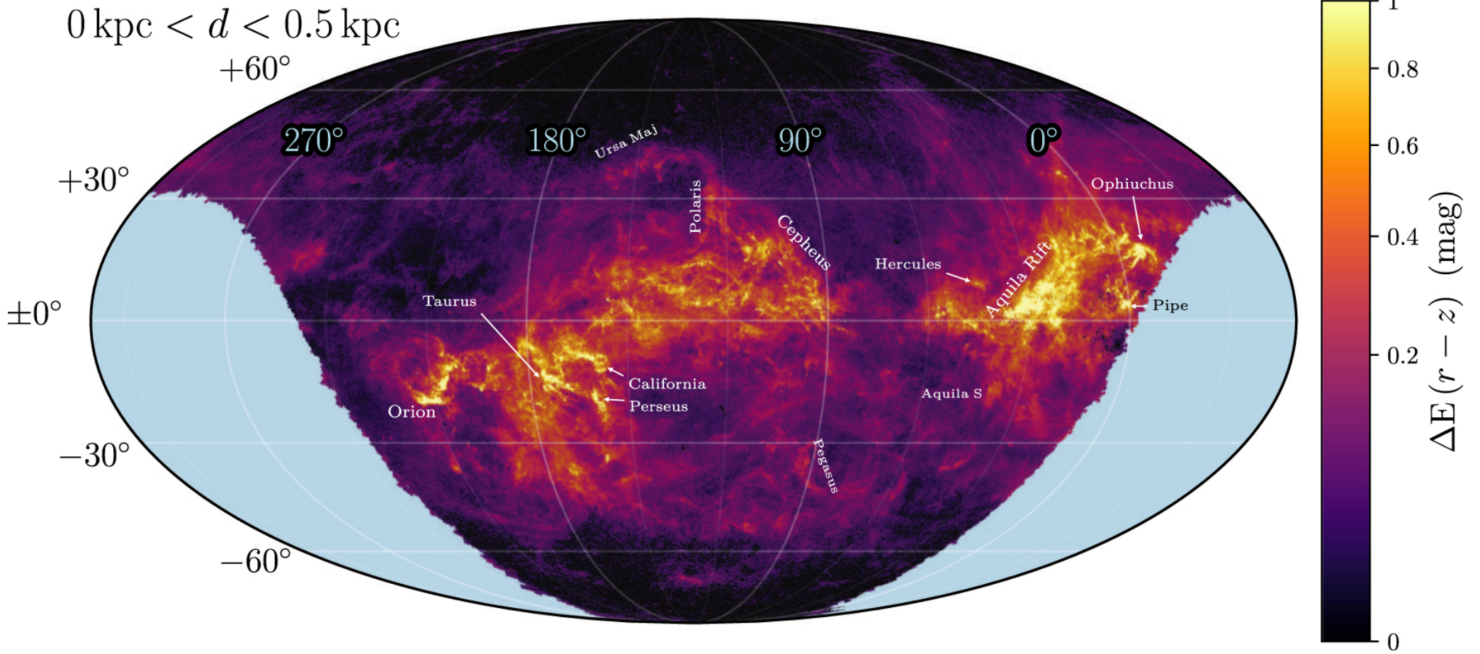
Figure 1. from A 3D Dust Map Based on Gaia, Pan-STARRS 1, and 2MASS null 2019 APJ 887 93 doi:10.3847/1538-4357/ab5362 http://dx.doi.org/10.3847/1538-4357/ab5362 © 2019. The American Astronomical Society. All rights reserved.
