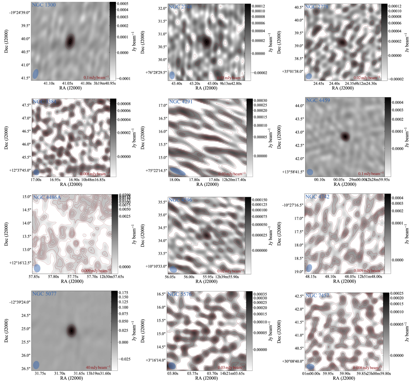
Figure 8. from The Fundamental Plane of Black Hole Accretion and Its Use as a Black Hole-Mass Estimator null 2019 APJ 871 80 doi:10.3847/1538-4357/aaf6b9 https://dx.doi.org/10.3847/1538-4357/aaf6b9 © 2019. The American Astronomical Society. All rights reserved.
