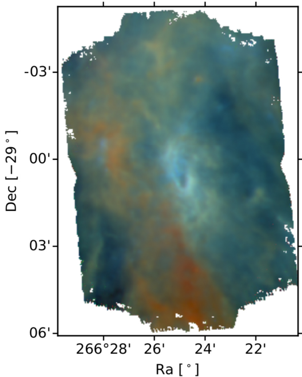
Figure 1. from A Detection of Sgr A* in the Far Infrared null 2018 APJ 862 129 doi:10.3847/1538-4357/aacd4b https://dx.doi.org/10.3847/1538-4357/aacd4b © 2018. The American Astronomical Society. All rights reserved.
