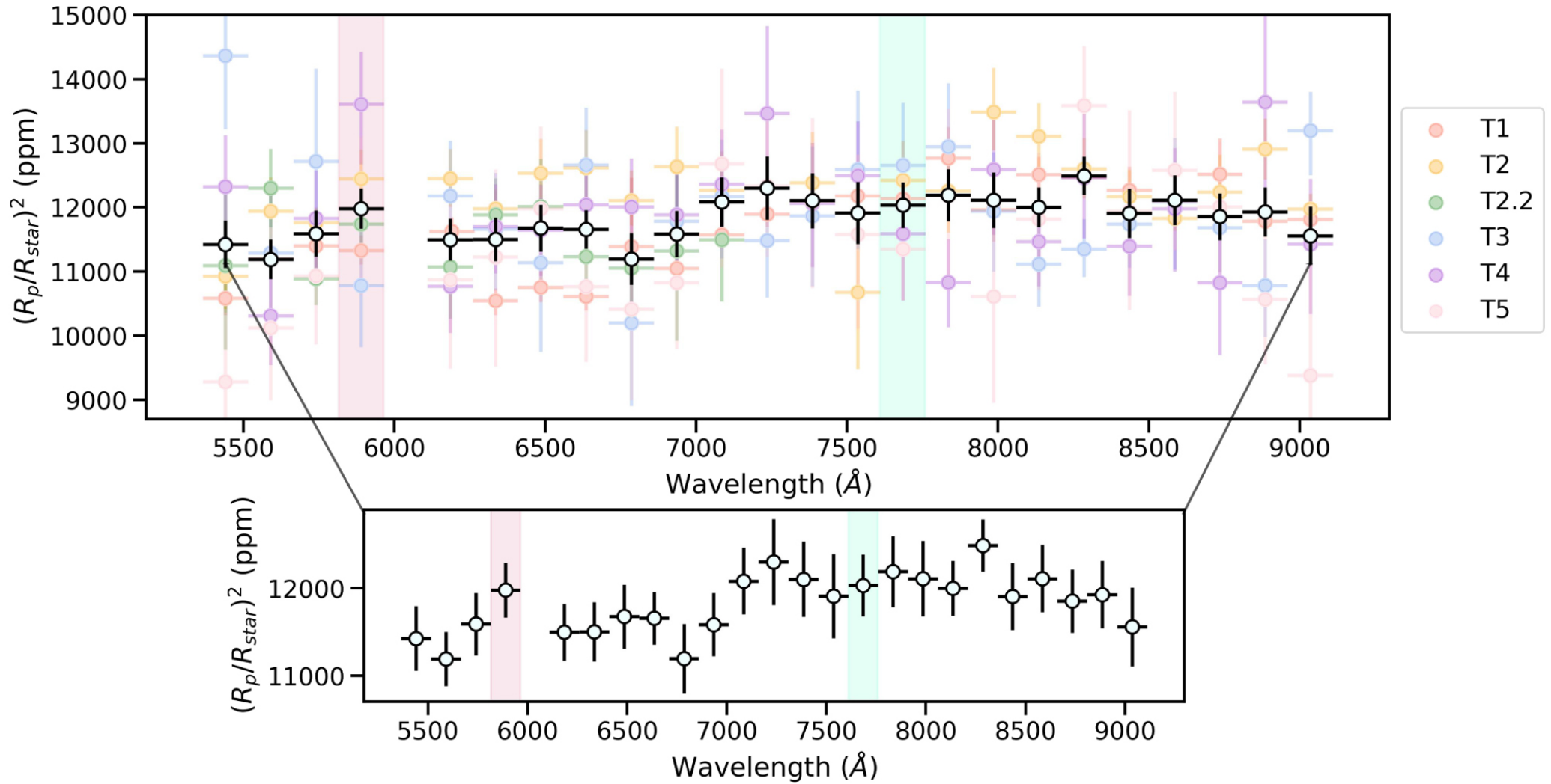
Figure 4. from Natalie H. Allen et al 2022 Astron. J. 164 doi:10.3847/1538-3881/ac8b74 http://dx.doi.org/10.3847/1538-3881/ac8b74 © 2022. The Author(s). Published by the American Astronomical Society.
