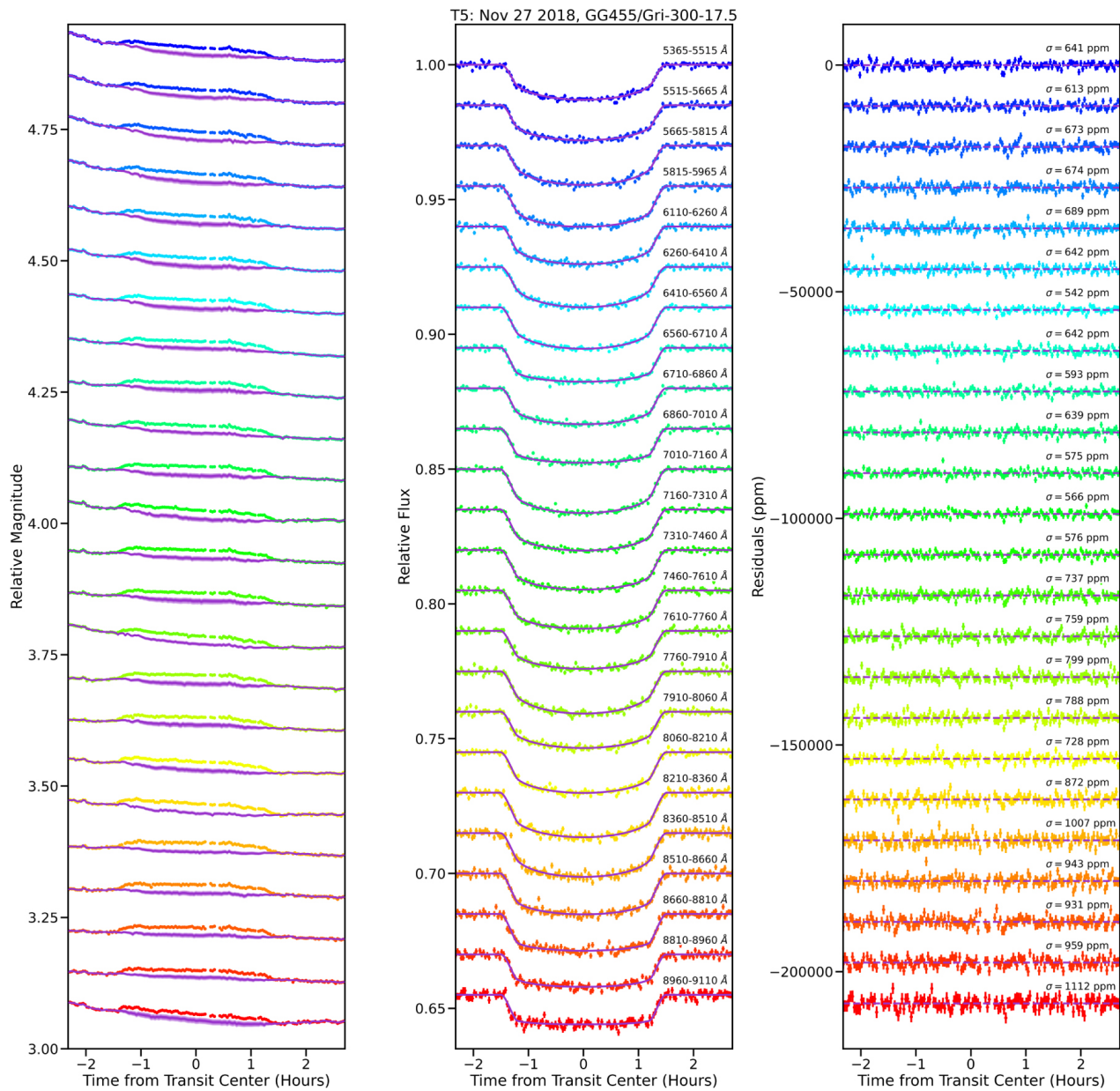
Figure 3. from Natalie H. Allen et al 2022 Astron. J. 164 doi:10.3847/1538-3881/ac8b74 https://dx.doi.org/10.3847/1538-3881/ac8b74 © 2022. The Author(s). Published by the American Astronomical Society.
