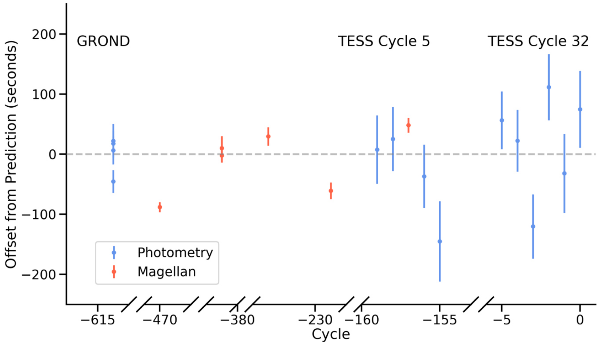
Figure 16. from Natalie H. Allen et al 2022 Astron. J. 164 doi:10.3847/1538-3881/ac8b74 https://dx.doi.org/10.3847/1538-3881/ac8b74 © 2022. The Author(s). Published by the American Astronomical Society.
