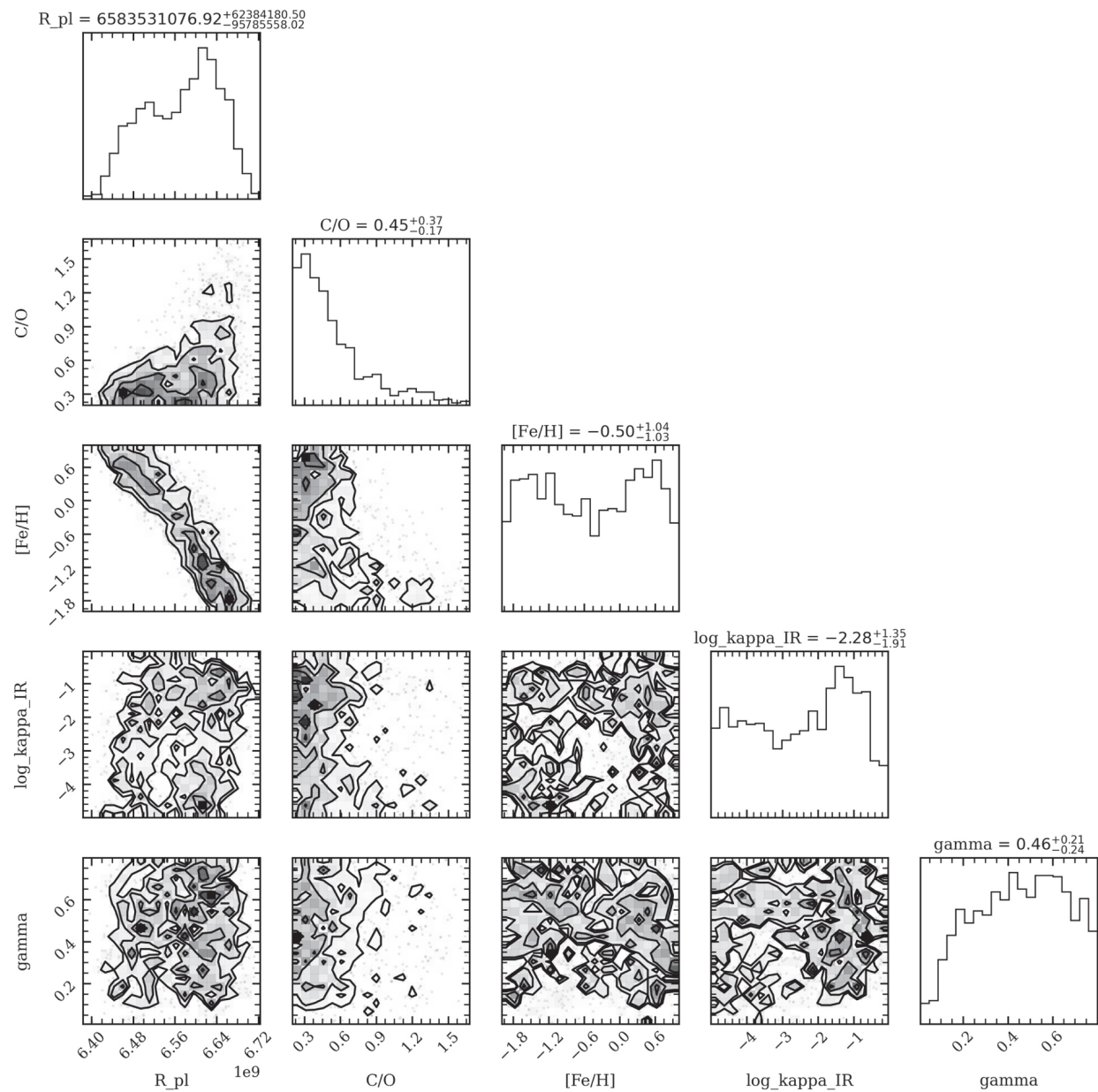
Figure 14. from Natalie H. Allen et al 2022 Astron. J. 164 doi:10.3847/1538-3881/ac8b74 https://dx.doi.org/10.3847/1538-3881/ac8b74 © 2022. The Author(s). Published by the American Astronomical Society.
