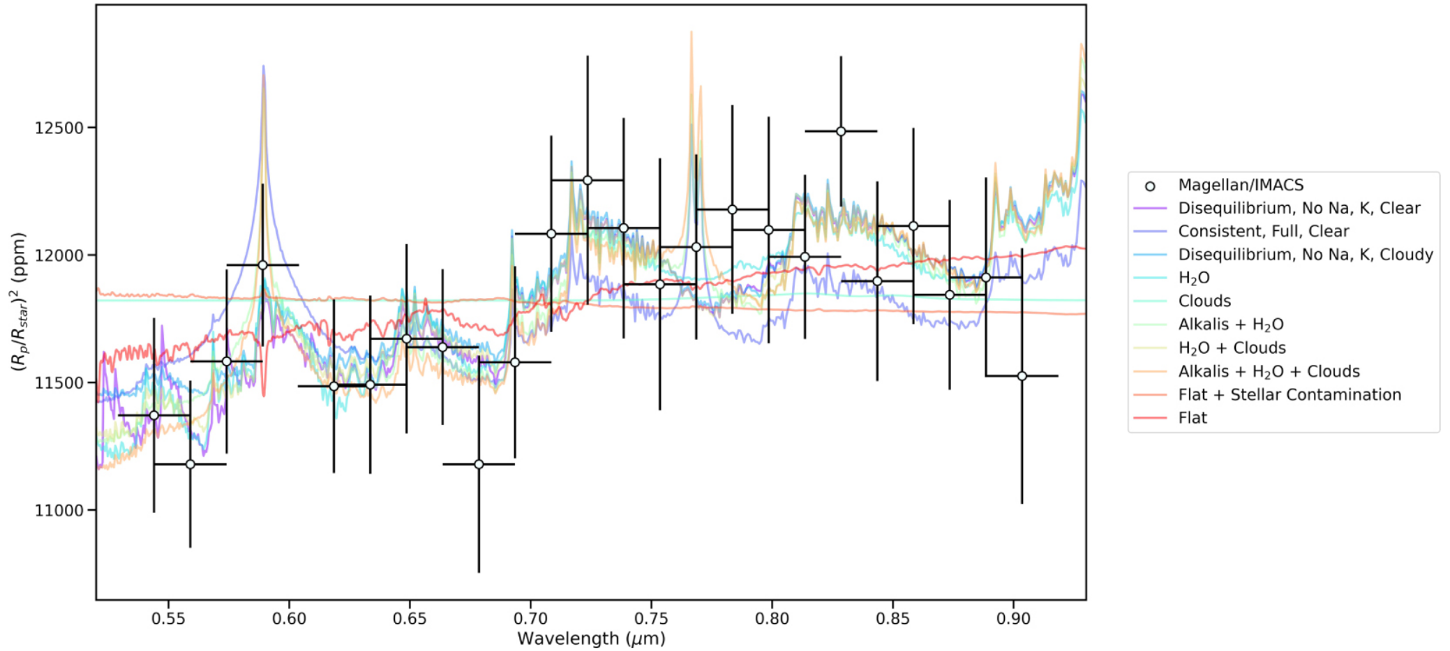
Figure 13. from Natalie H. Allen et al 2022 Astron. J. 164 doi:10.3847/1538-3881/ac8b74 http://dx.doi.org/10.3847/1538-3881/ac8b74 © 2022. The Author(s). Published by the American Astronomical Society.
