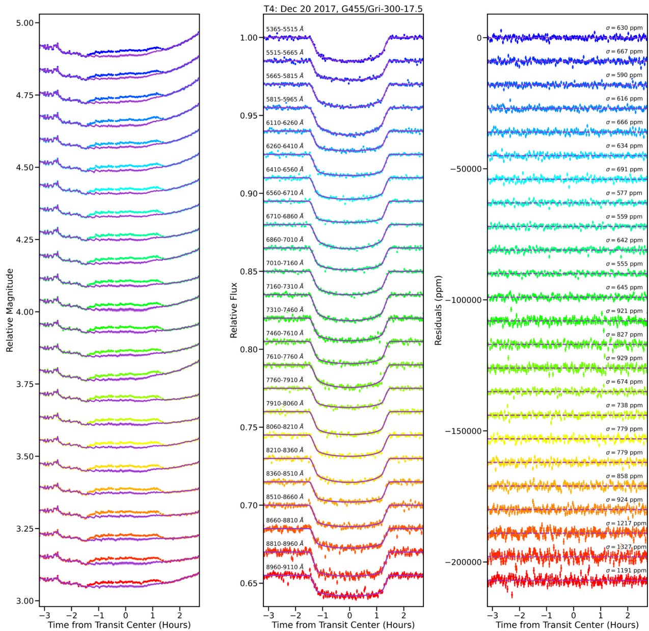
Figure 12. from Natalie H. Allen et al 2022 Astron. J. 164 doi:10.3847/1538-3881/ac8b74 https://dx.doi.org/10.3847/1538-3881/ac8b74 © 2022. The Author(s). Published by the American Astronomical Society.
