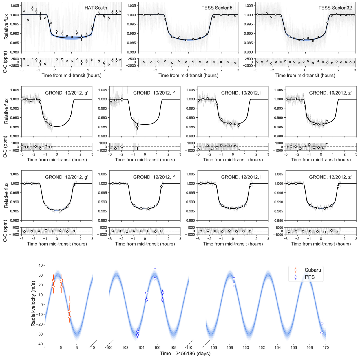
Figure 1. from Natalie H. Allen et al 2022 Astron. J. 164 doi:10.3847/1538-3881/ac8b74 https://dx.doi.org/10.3847/1538-3881/ac8b74 © 2022. The Author(s). Published by the American Astronomical Society.
