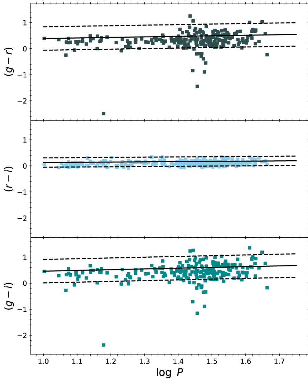
Figure 8. from Chow-Choong Ngeow et al 2022 Astron. J. 164 doi:10.3847/1538-3881/ac87a4 https://dx.doi.org/10.3847/1538-3881/ac87a4 © 2022. The Author(s). Published by the American Astronomical Society.
