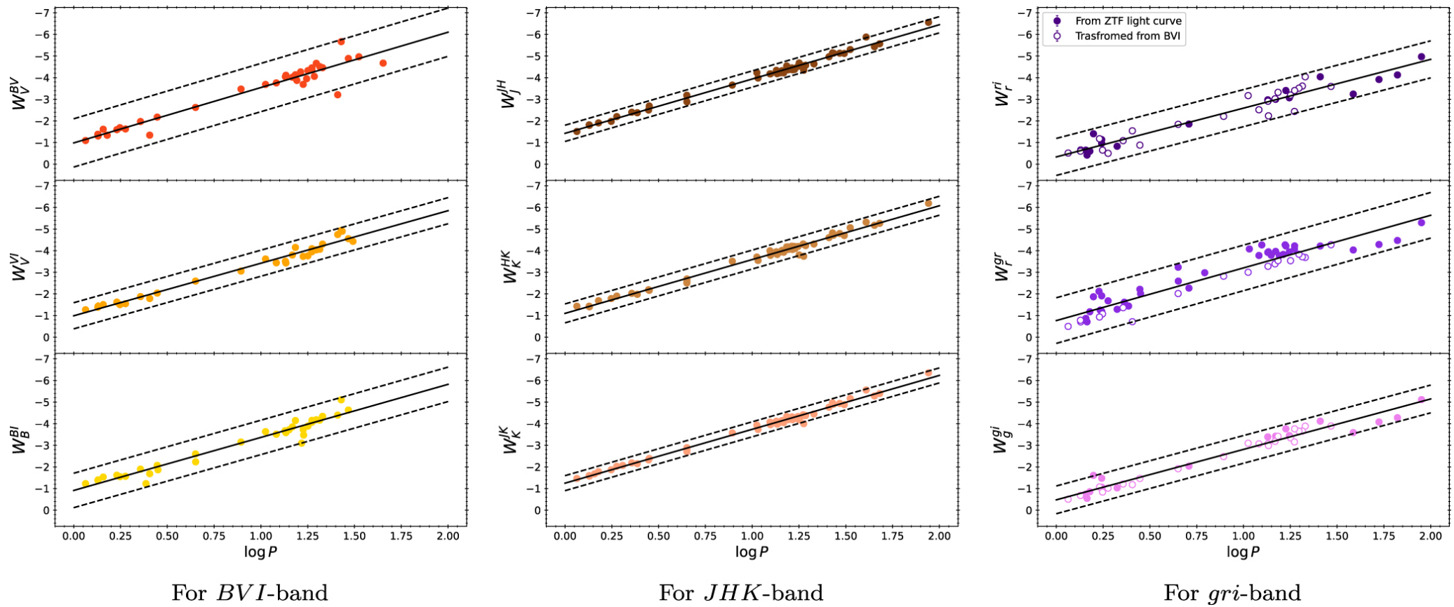
Figure 6. from Chow-Choong Ngeow et al 2022 Astron. J. 164 doi:10.3847/1538-3881/ac87a4 https://dx.doi.org/10.3847/1538-3881/ac87a4 © 2022. The Author(s). Published by the American Astronomical Society.
