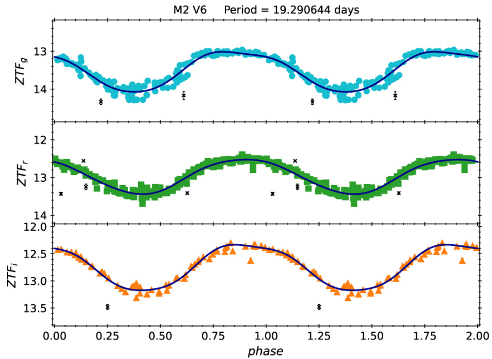
Figure 1. from Chow-Choong Ngeow et al 2022 Astron. J. 164 doi:10.3847/1538-3881/ac87a4 https://dx.doi.org/10.3847/1538-3881/ac87a4 © 2022. The Author(s). Published by the American Astronomical Society.
