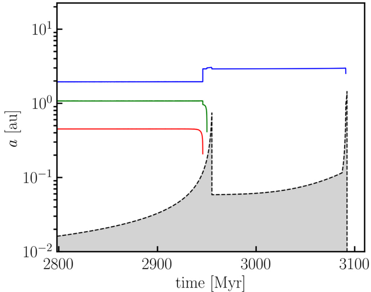
Figure 7. from Trifon Trifonov et al 2022 Astron. J. 164 doi:10.3847/1538-3881/ac7ce0 https://dx.doi.org/10.3847/1538-3881/ac7ce0 © 2022. The Author(s). Published by the American Astronomical Society.
