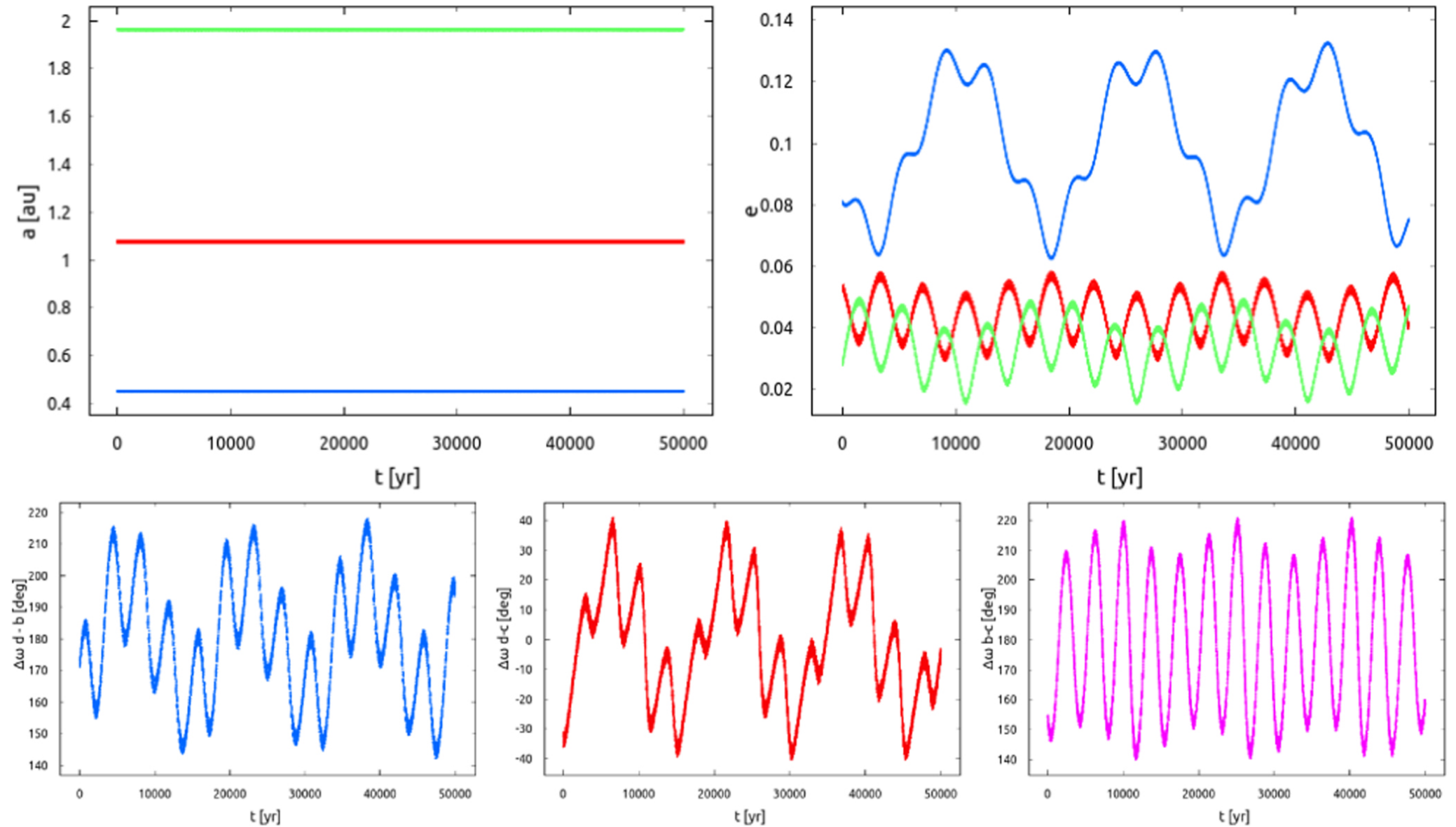
Figure 5. from Trifon Trifonov et al 2022 Astron. J. 164 doi:10.3847/1538-3881/ac7ce0 https://dx.doi.org/10.3847/1538-3881/ac7ce0 © 2022. The Author(s). Published by the American Astronomical Society.
