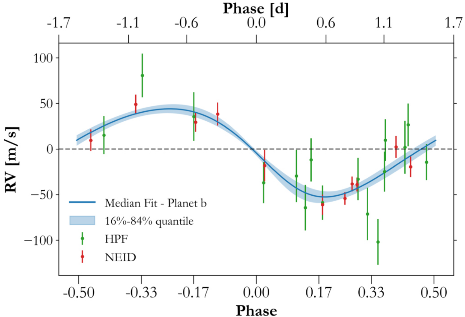
Figure 7. from Shubham Kanodia et al 2022 Astron. J. 164 doi:10.3847/1538-3881/ac7c20 http://dx.doi.org/10.3847/1538-3881/ac7c20 © 2022. The Author(s). Published by the American Astronomical Society.
