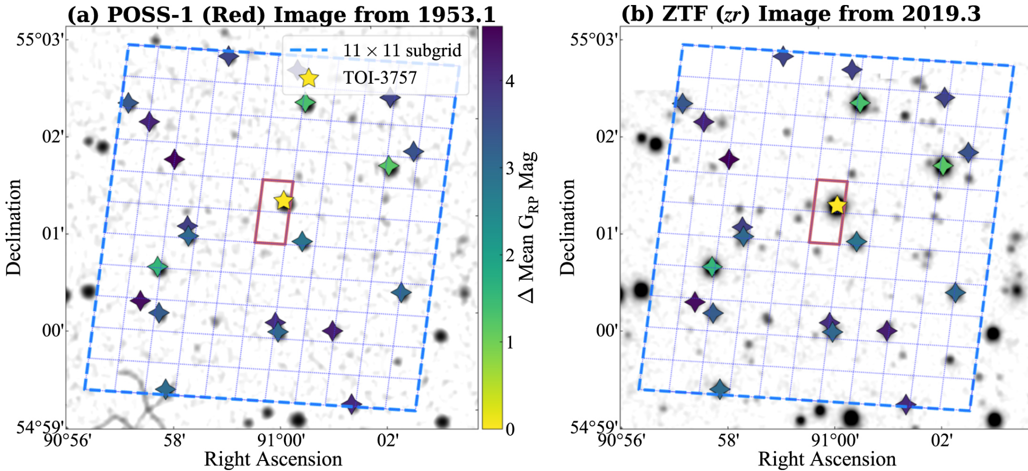
Figure 5. from Shubham Kanodia et al 2022 Astron. J. 164 doi:10.3847/1538-3881/ac7c20 http://dx.doi.org/10.3847/1538-3881/ac7c20 © 2022. The Author(s). Published by the American Astronomical Society.
