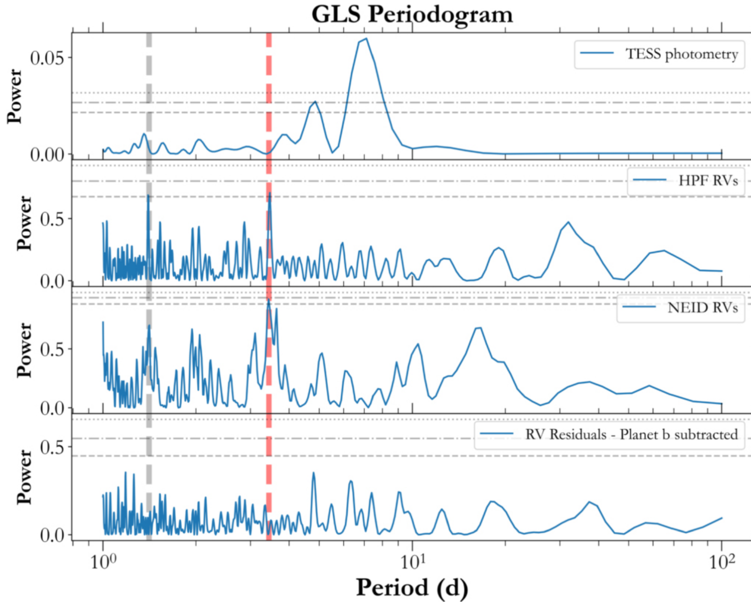
Figure 4. from Shubham Kanodia et al 2022 Astron. J. 164 doi:10.3847/1538-3881/ac7c20 http://dx.doi.org/10.3847/1538-3881/ac7c20 © 2022. The Author(s). Published by the American Astronomical Society.
