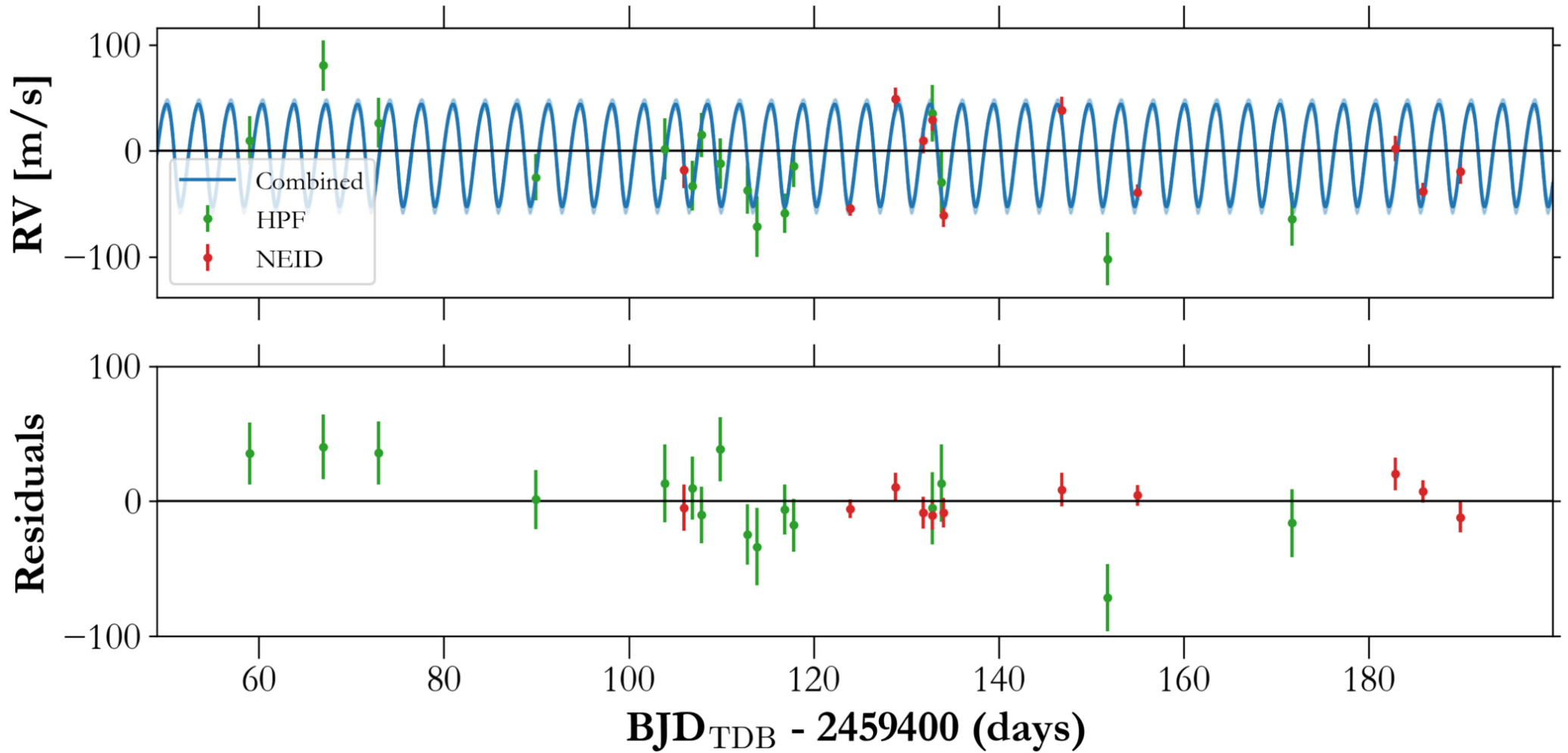
Figure 3. from Shubham Kanodia et al 2022 Astron. J. 164 doi:10.3847/1538-3881/ac7c20 http://dx.doi.org/10.3847/1538-3881/ac7c20 © 2022. The Author(s). Published by the American Astronomical Society.
