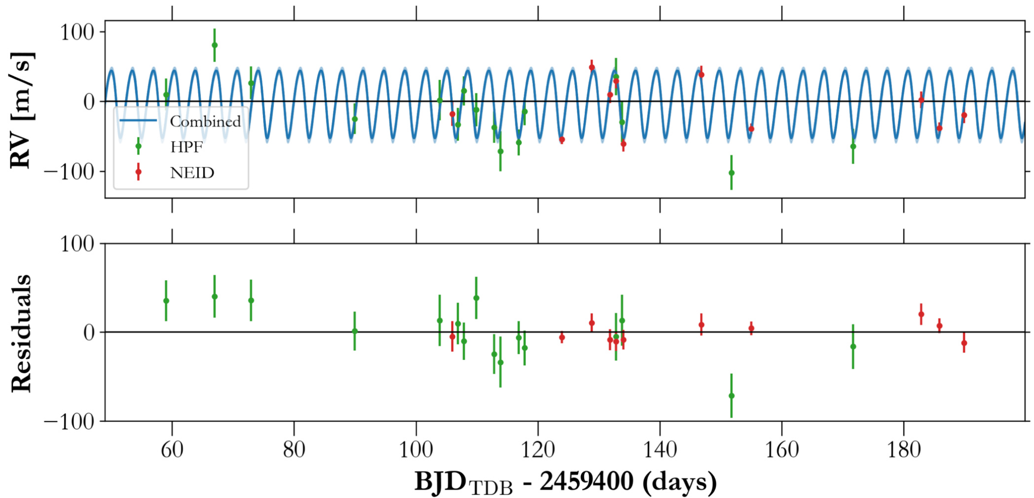
Figure 3. from Shubham Kanodia et al 2022 Astron. J. 164 doi:10.3847/1538-3881/ac7c20 https://dx.doi.org/10.3847/1538-3881/ac7c20 © 2022. The Author(s). Published by the American Astronomical Society.
