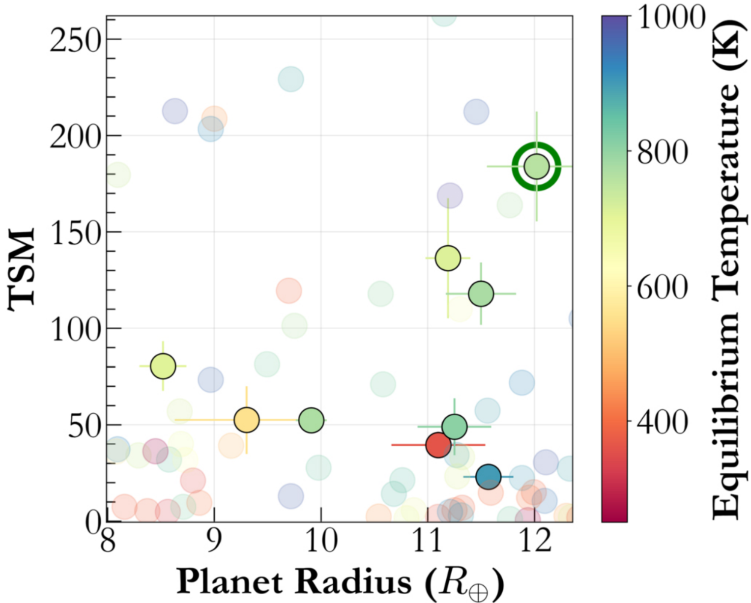
Figure 11. from Shubham Kanodia et al 2022 Astron. J. 164 doi:10.3847/1538-3881/ac7c20 http://dx.doi.org/10.3847/1538-3881/ac7c20 © 2022. The Author(s). Published by the American Astronomical Society.
