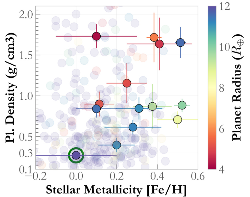
b) Planet density as a function of stellar metallicity
