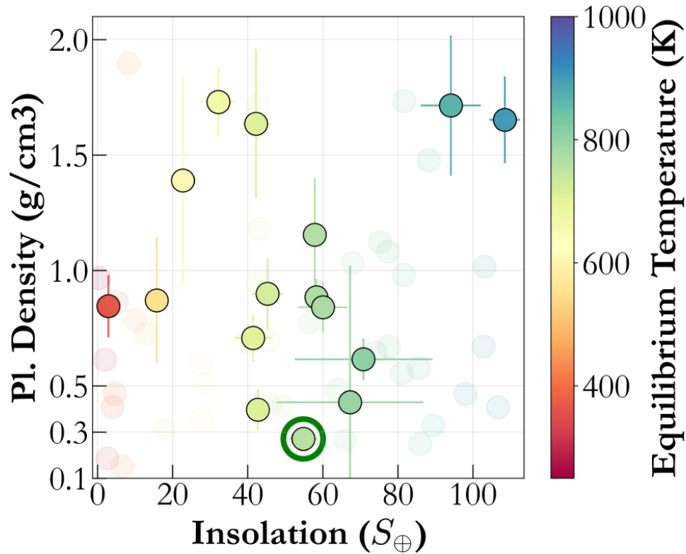
a) Planet density as a function of insolation flux
