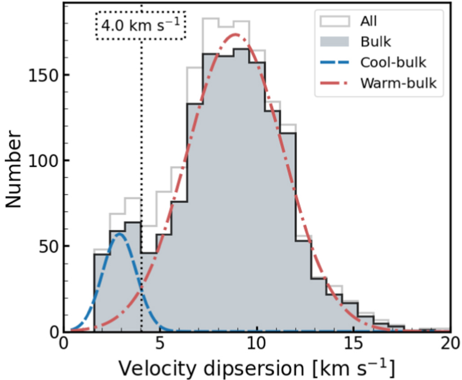
Figure 8. from Hye-Jin Park et al 2022 Astron. J. 164 doi:10.3847/1538-3881/ac7c1b http://dx.doi.org/10.3847/1538-3881/ac7c1b © 2022. The Author(s). Published by the American Astronomical Society.
