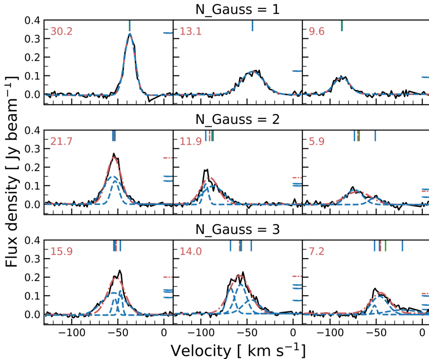
Figure 4. from Hye-Jin Park et al 2022 Astron. J. 164 doi:10.3847/1538-3881/ac7c1b https://dx.doi.org/10.3847/1538-3881/ac7c1b © 2022. The Author(s). Published by the American Astronomical Society.
