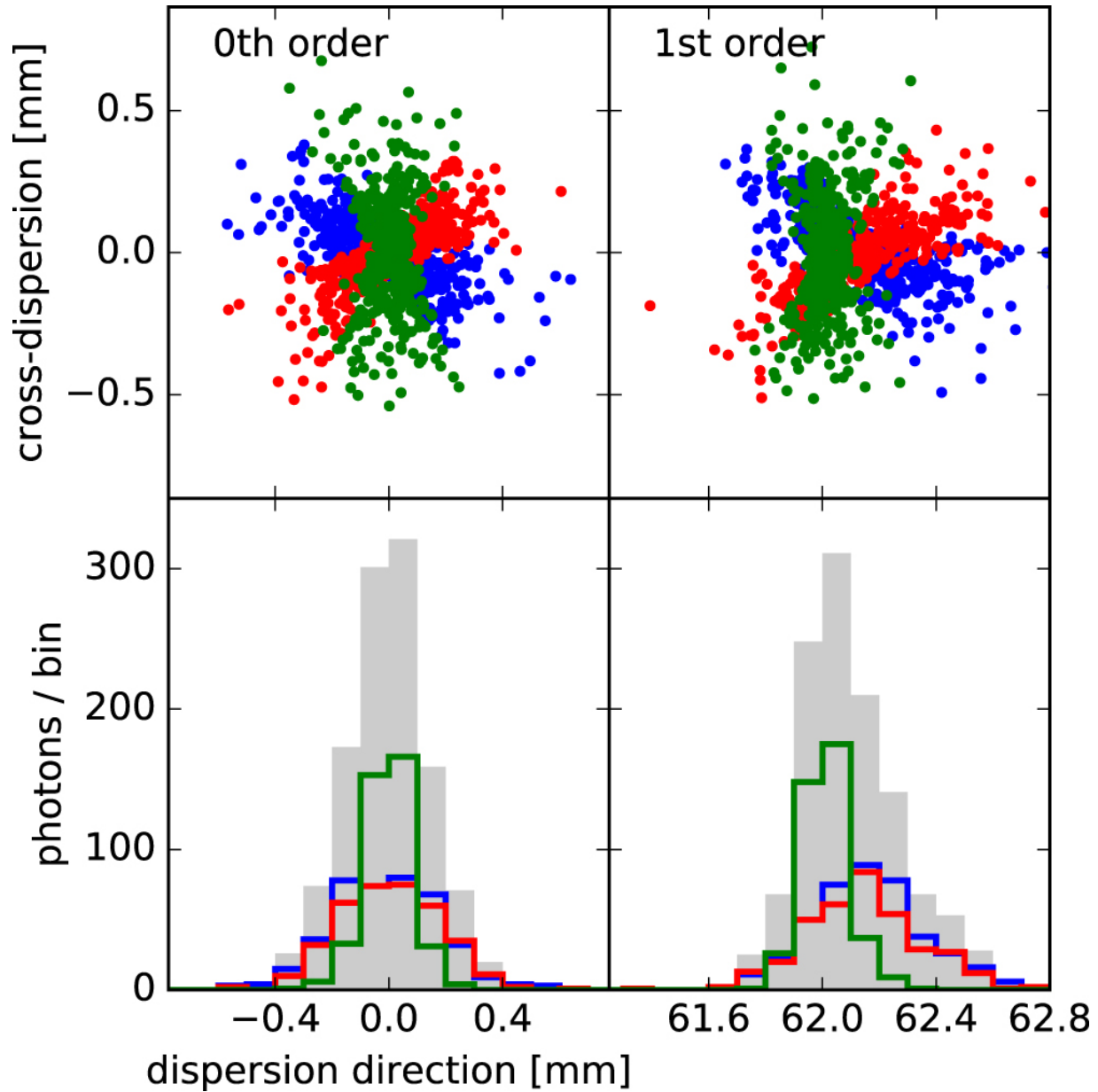
Figure 2. from MARXS: A Modular Software to Ray-trace X-Ray Instrumentation null 2017 AJ 154 243 doi:10.3847/1538-3881/aa943b https://dx.doi.org/10.3847/1538-3881/aa943b © 2017. The American Astronomical Society. All rights reserved.
