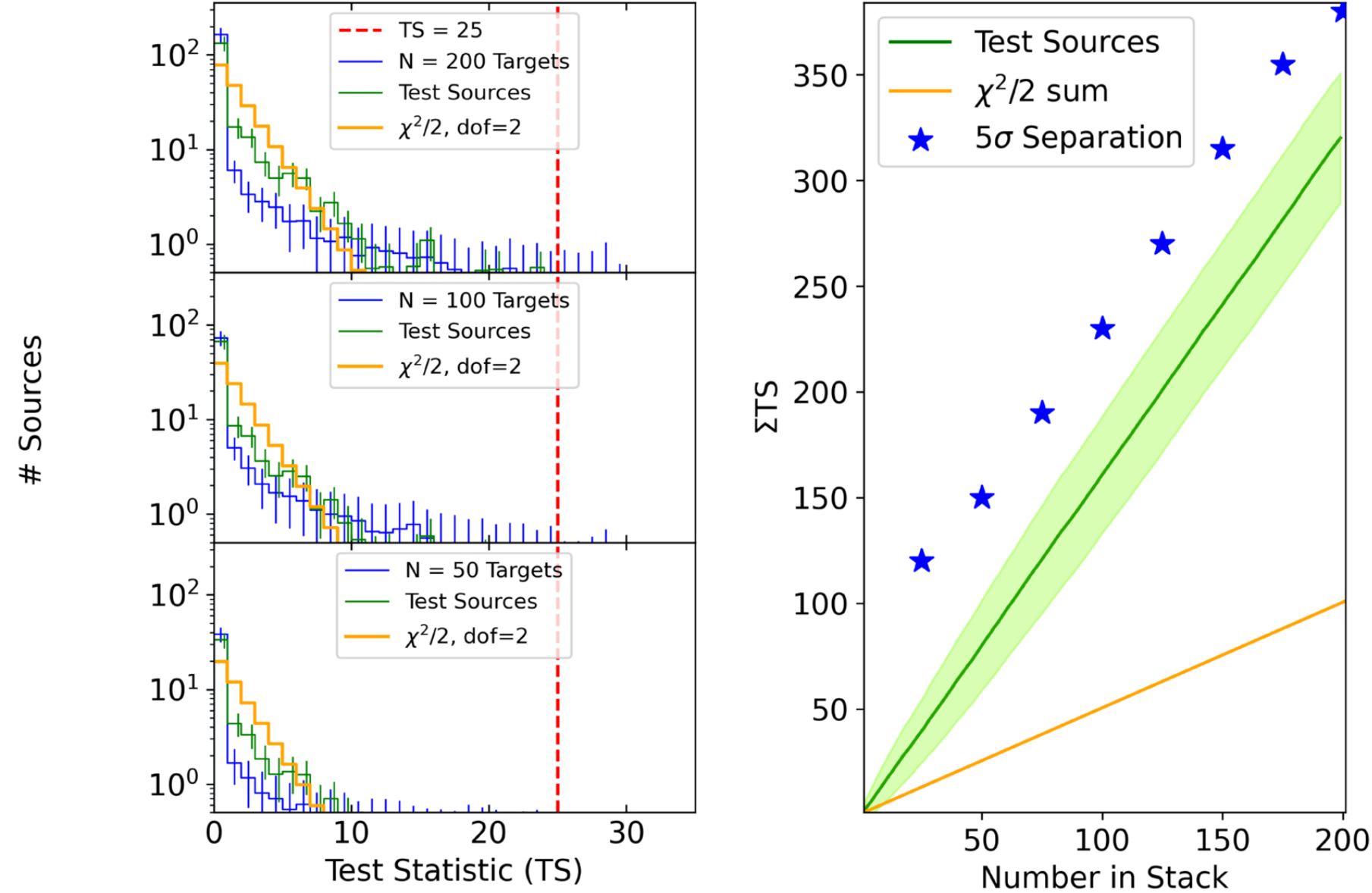
Figure 1. from Owen K. Henry et al 2026 Res. Notes AAS 10 doi:10.3847/2515-5172/aeb6e5 https://dx.doi.org/10.3847/2515-5172/aeb6e5 © 2026. The Author(s). Published by the American Astronomical Society.
