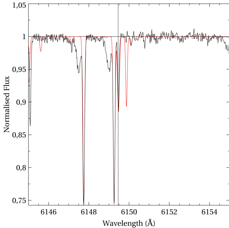
Figure 1. from Richard Monier 2026 Res. Notes AAS 10 doi:10.3847/2515-5172/aeaed3 https://dx.doi.org/10.3847/2515-5172/aeaed3 © 2026. The Author(s). Published by the American Astronomical Society.
