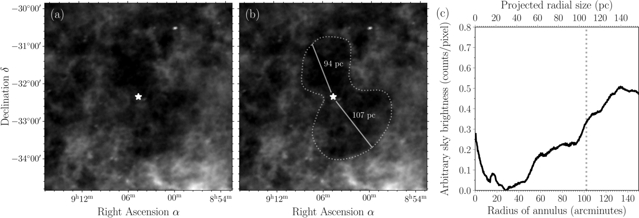
Figure 1. from Michael W. Healy-Kalesh and Matthew J. Darnley 2026 Res. Notes AAS 10 doi:10.3847/2515-5172/aeab95 https://dx.doi.org/10.3847/2515-5172/aeab95 © 2026. The Author(s). Published by the American Astronomical Society.
