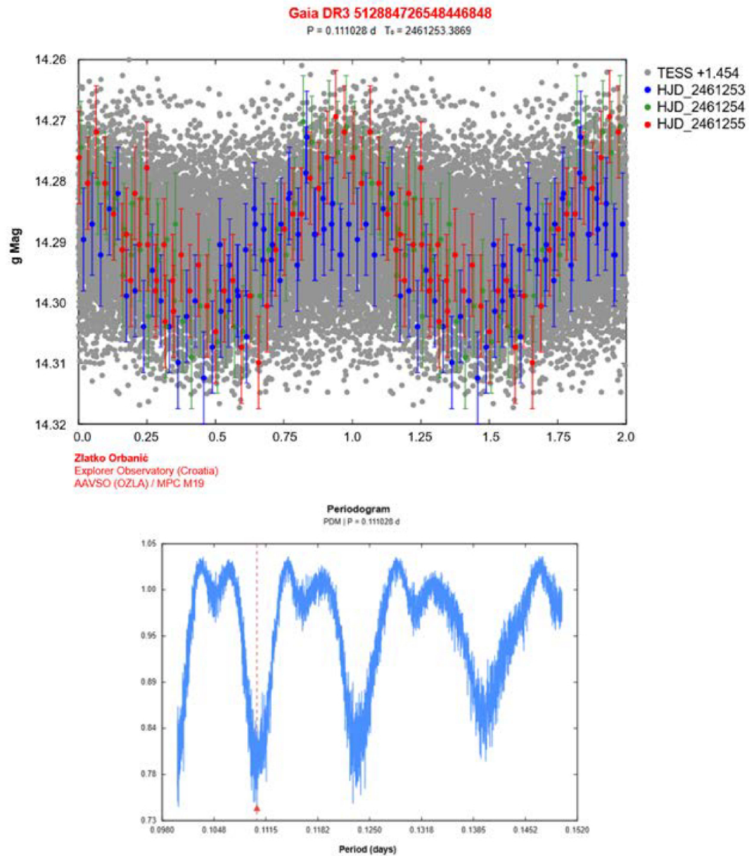
Figure 1. from Zlatko Orbanic 2026 Res. Notes AAS 10 doi:10.3847/2515-5172/aea995 https://dx.doi.org/10.3847/2515-5172/aea995 © 2026. The Author(s). Published by the American Astronomical Society.
