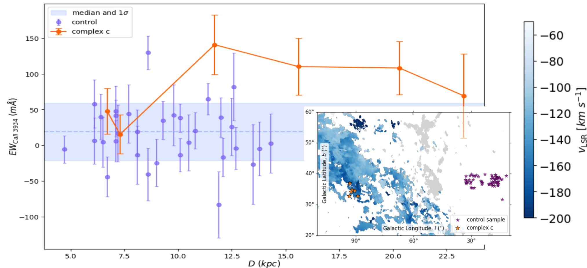
Figure 1. from Annabelle Lin et al 2026 Res. Notes AAS 10 doi:10.3847/2515-5172/aea98a https://dx.doi.org/10.3847/2515-5172/aea98a © 2026. The Author(s). Published by the American Astronomical Society.
