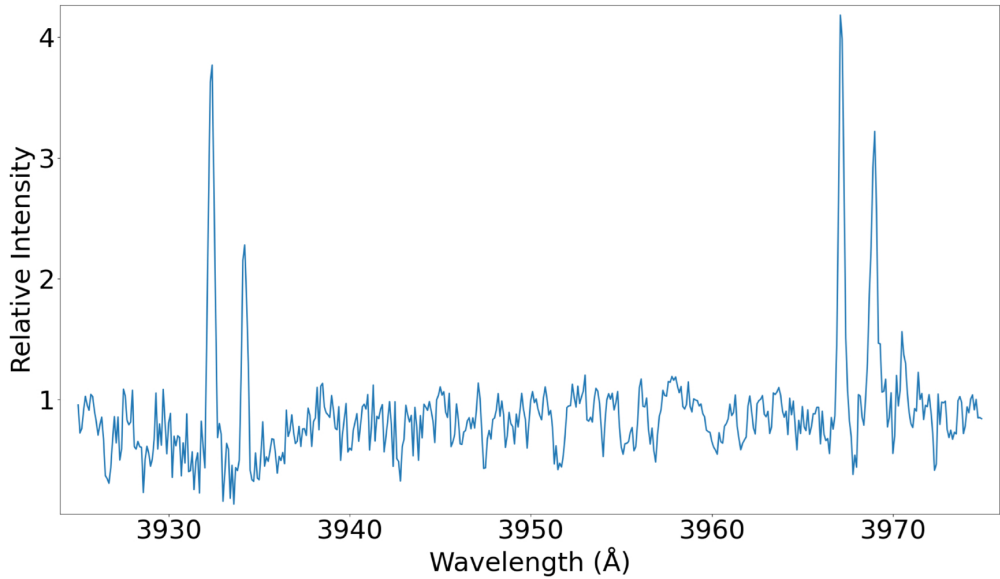
Figure 1. from Tamara A. S. Bleeker et al 2026 Res. Notes AAS 10 doi:10.3847/2515-5172/aea8ed https://dx.doi.org/10.3847/2515-5172/aea8ed © 2026. The Author(s). Published by the American Astronomical Society.
