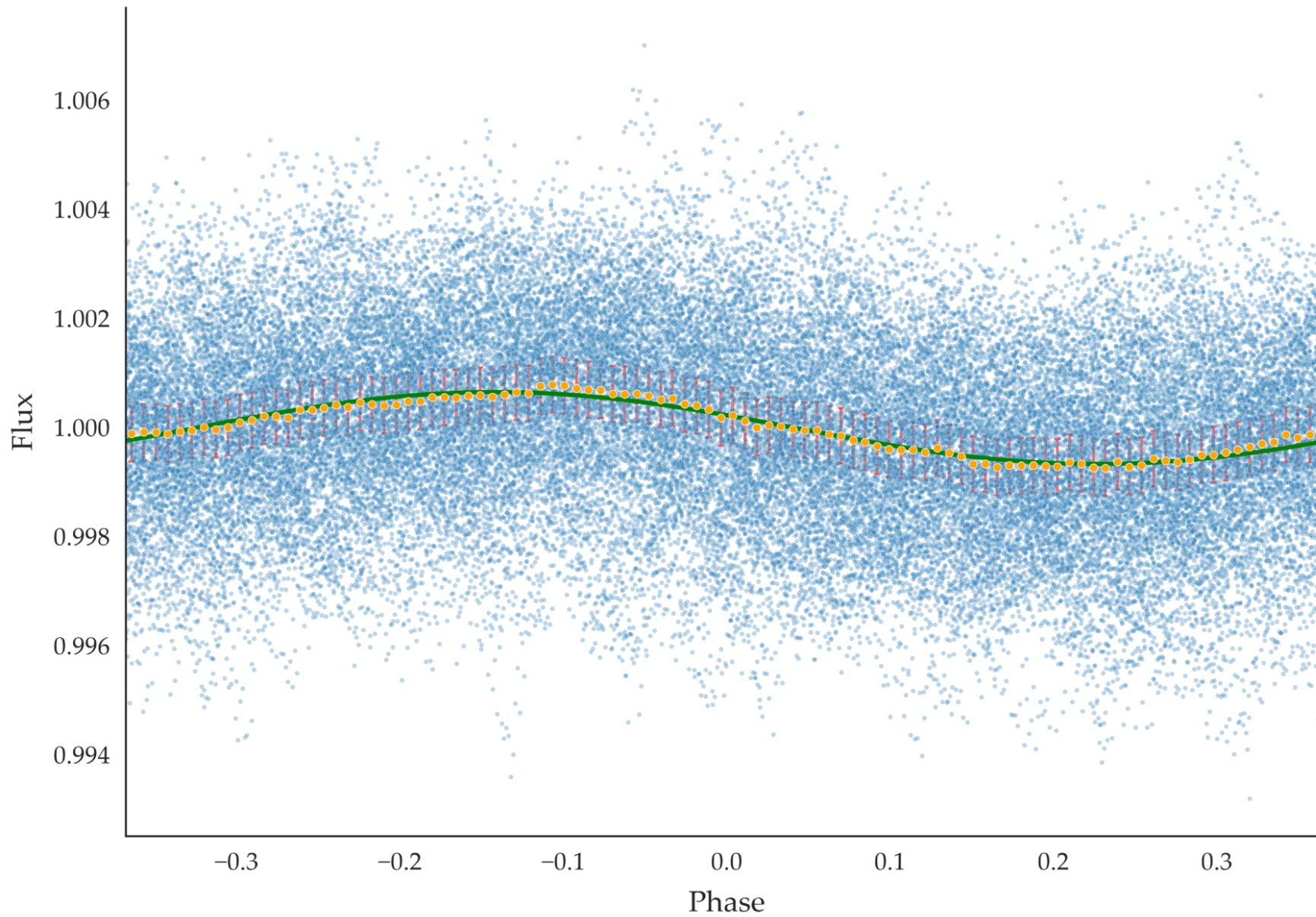
Figure 1. from Adam McMaster et al 2026 Res. Notes AAS 10 doi:10.3847/2515-5172/aea61f https://dx.doi.org/10.3847/2515-5172/aea61f © 2026. The Author(s). Published by the American Astronomical Society.
