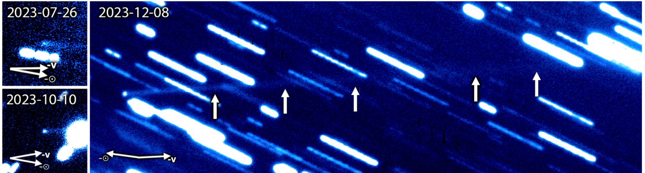
Figure 1. from Henry H. Hsieh et al 2026 Res. Notes AAS 10 doi:10.3847/2515-5172/aea5ff https://dx.doi.org/10.3847/2515-5172/aea5ff © 2026. The Author(s). Published by the American Astronomical Society.
