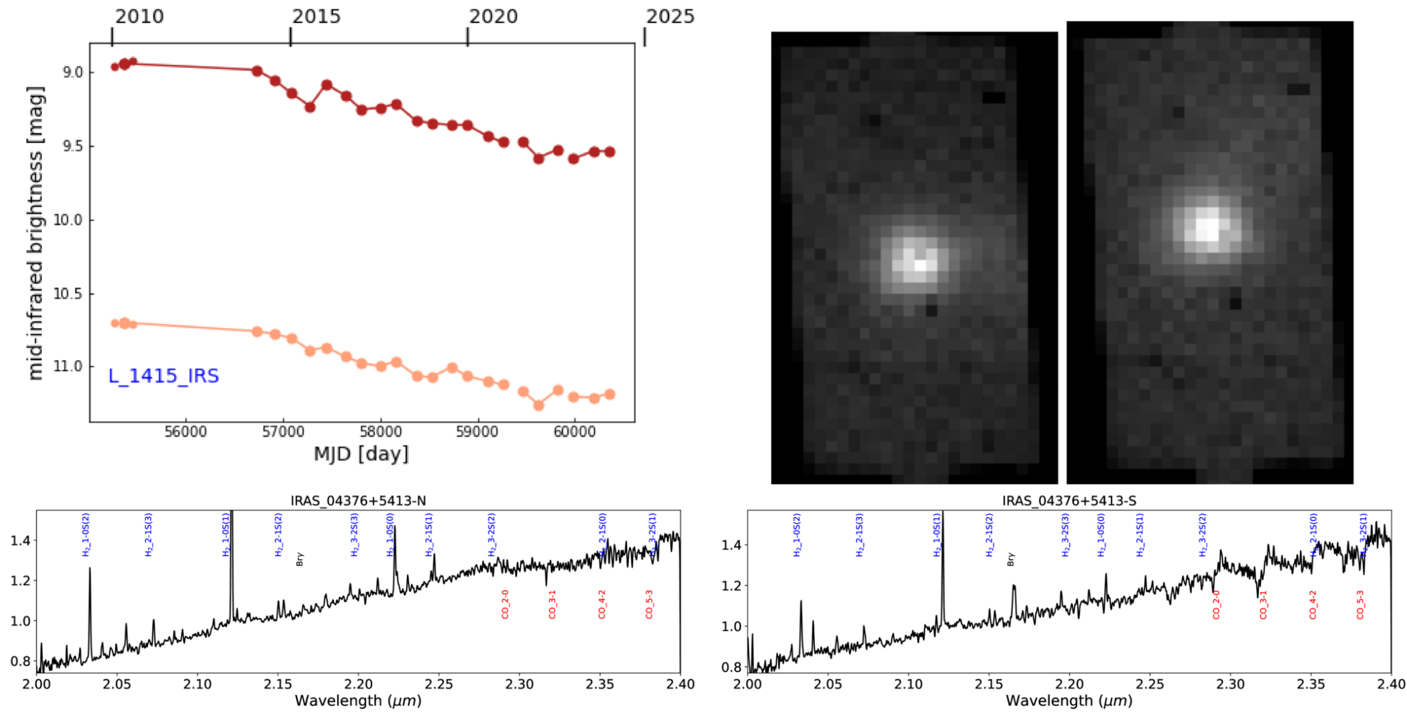
Figure 1. from Lynne A. Hillenbrand et al 2026 Res. Notes AAS 10 doi:10.3847/2515-5172/aea5fe https://dx.doi.org/10.3847/2515-5172/aea5fe © 2026. The Author(s). Published by the American Astronomical Society.
